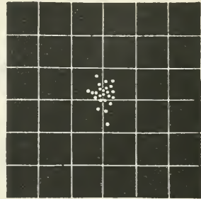
Diagram of 24 Shots at 30 Yards' Distance, made at Woolwich with this Revolver at a target 6ft. square.
